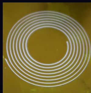
Silver Paste Coil on Kapton
